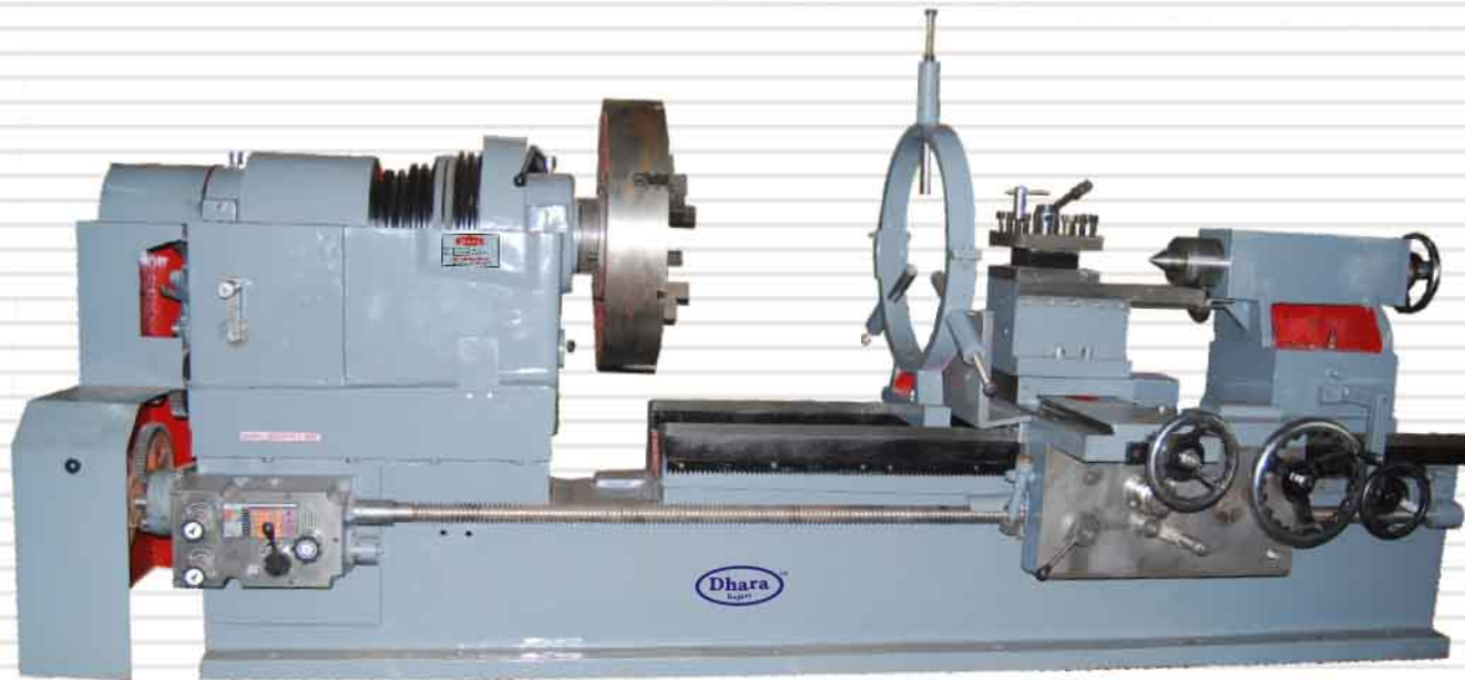
Extra Heavy Duty Plano Type Lathe Machine
